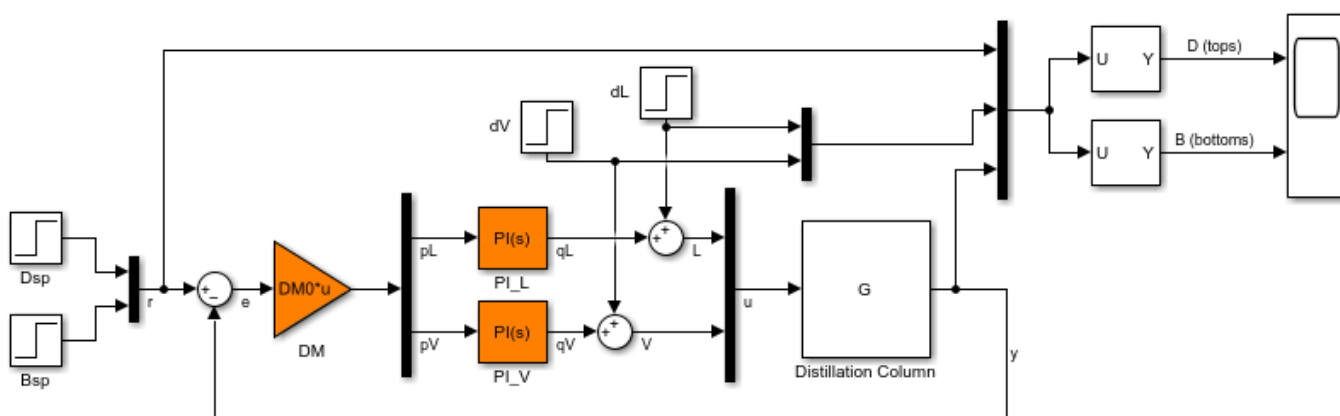
Decoupling controller for a distillation column
